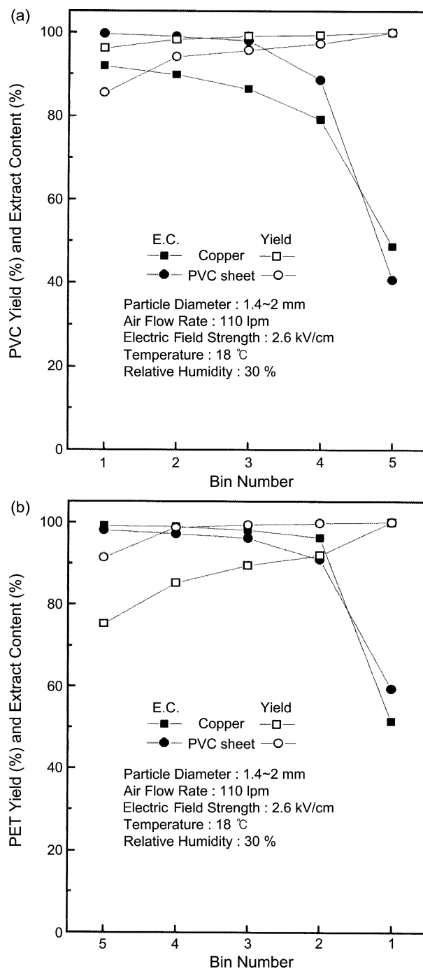
Fig. 9. Extract content and yield of PVC/PET as function of tribocharger materials [(a) Copper, (b) PVC sheet].
